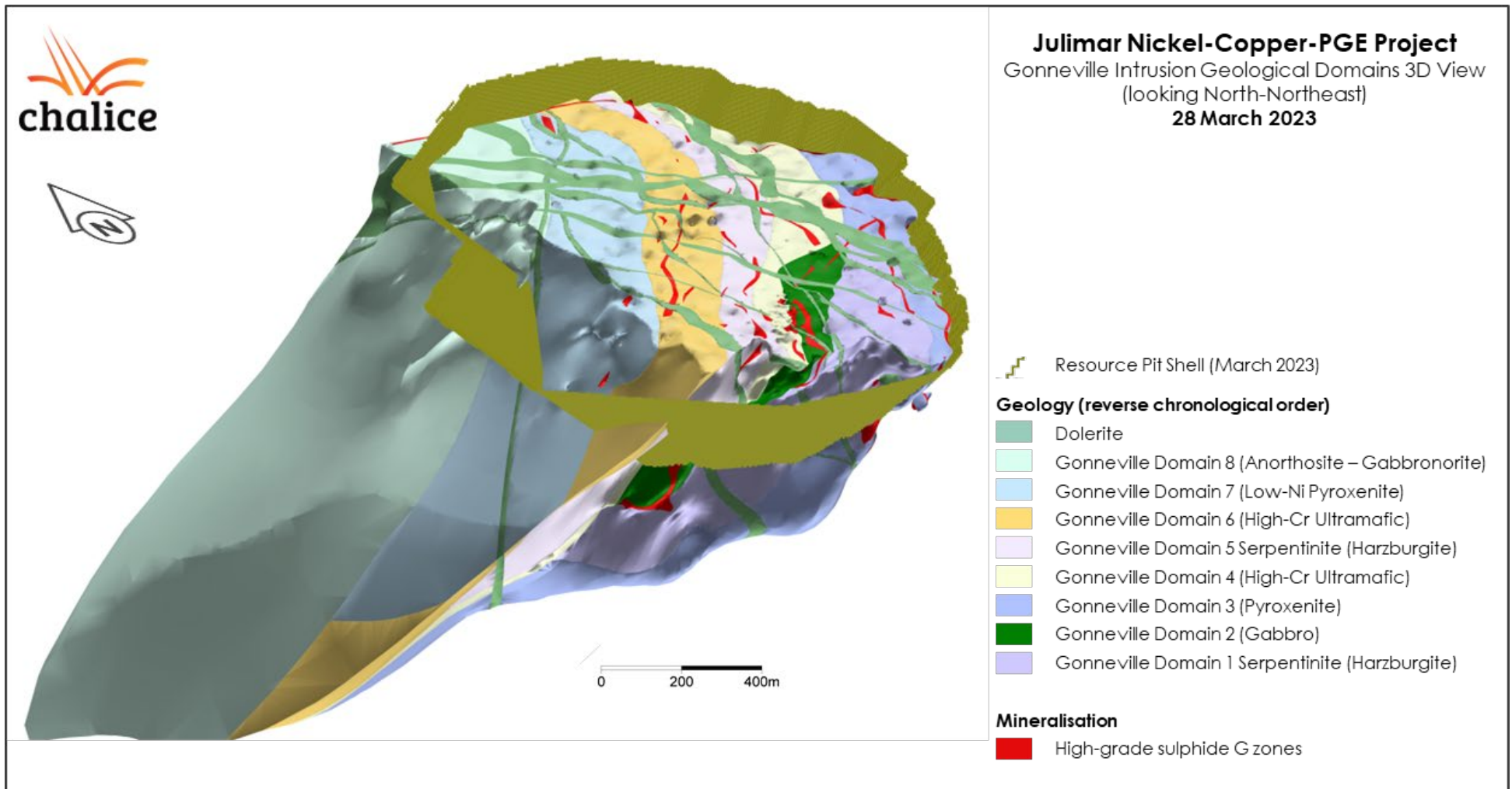
Figure 6. Gonneville 3D view (looking NNE) – local geology and resource pit shell.
