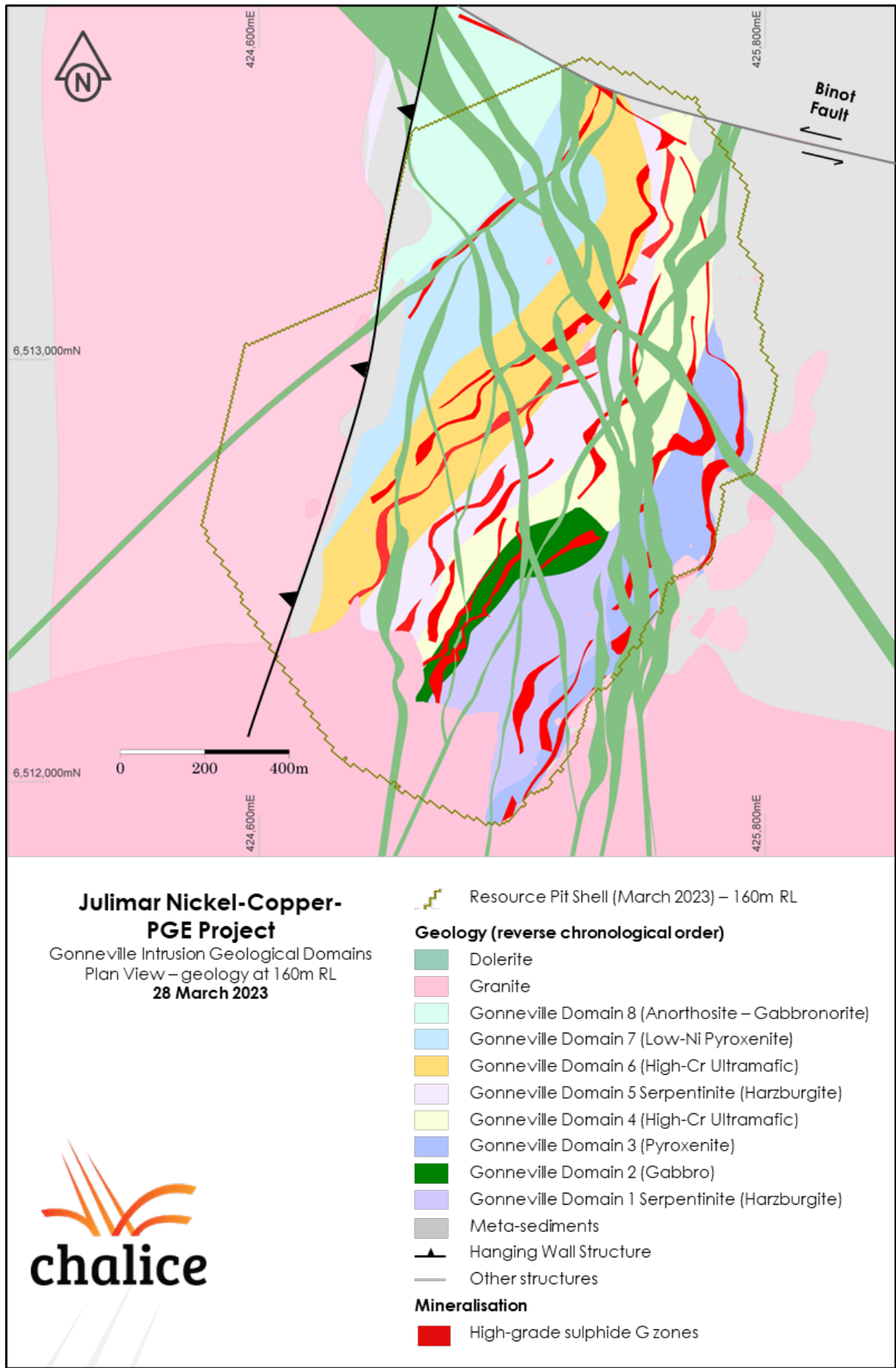
Figure 7. Gonneville Plan View – local geology and resource pit outline at depth of ~80m.
