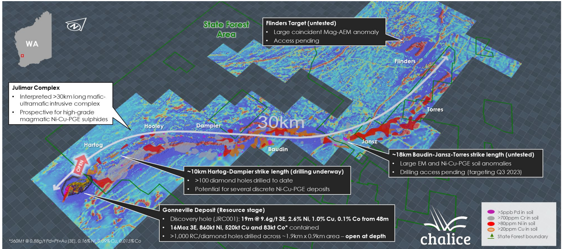
Figure 8. Julimar Complex 3D View (looking NW) – Gonneville Deposit, targets, soil geochemistry over regional magnetics.
