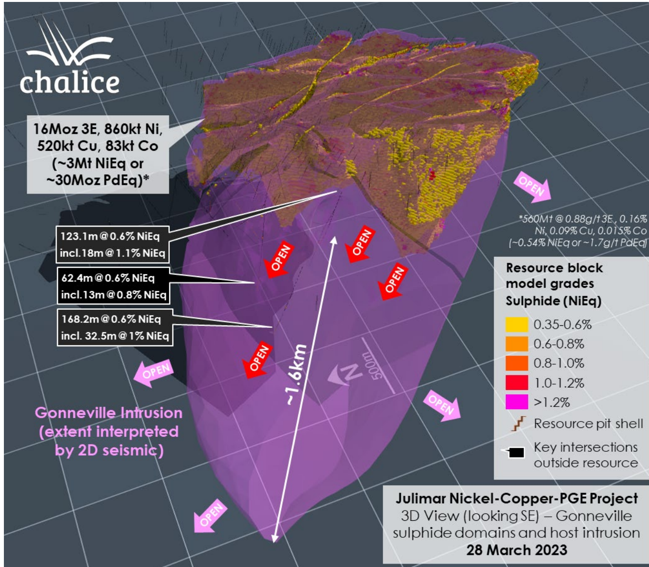
Figure 7. 3D view (looking SE) of Gonneville sulphide block model and host intrusion.
