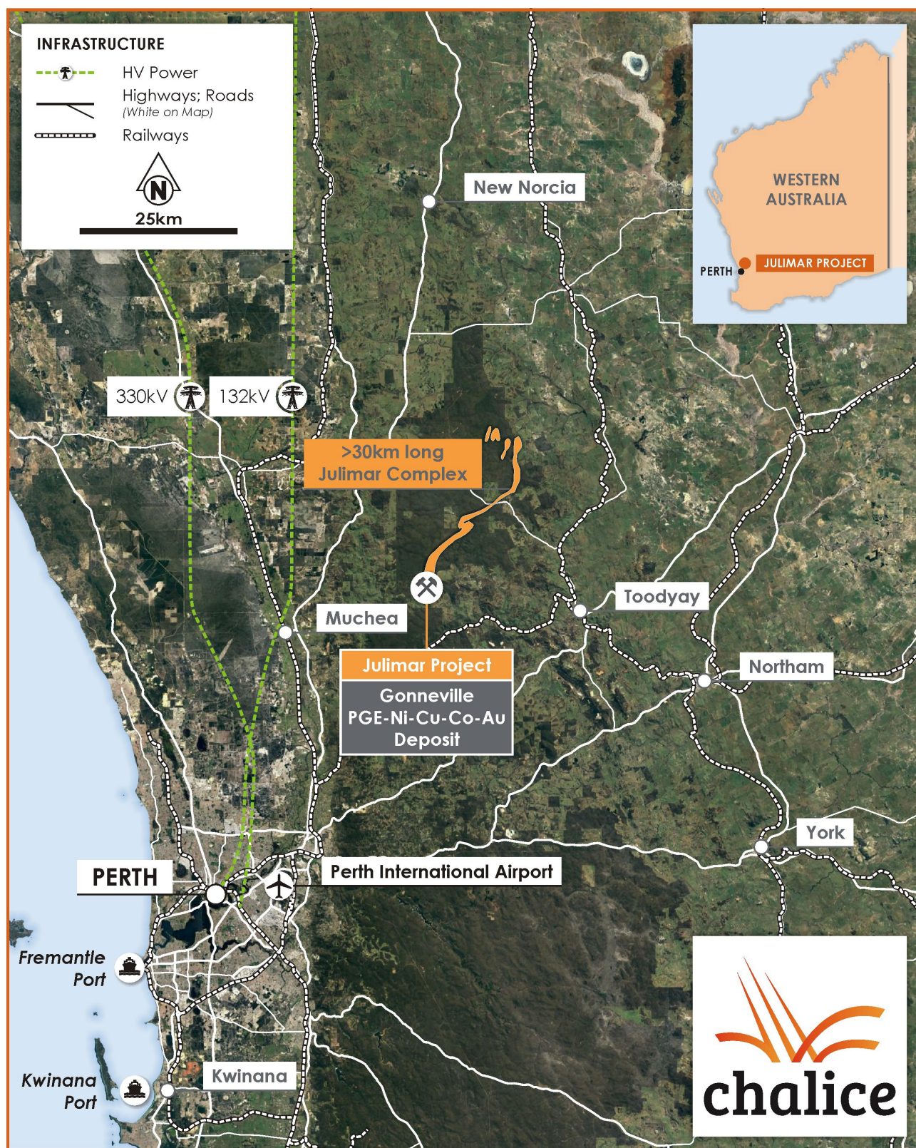
Figure 2. Julimar Complex, Gonneville Deposit, Project tenure and nearby infrastructure.
