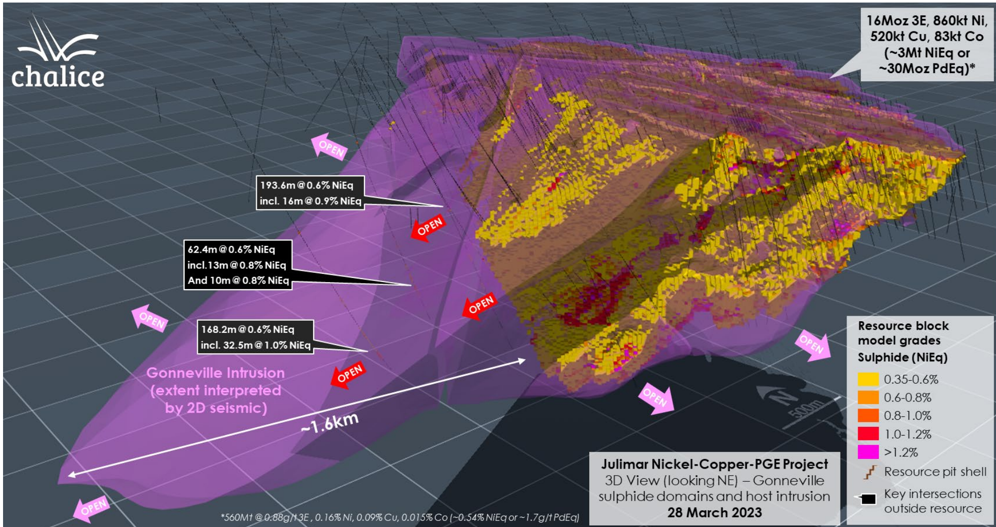
Figure 6. 3D view (looking NE) of Gonneville sulphide block model and host intrusion.
