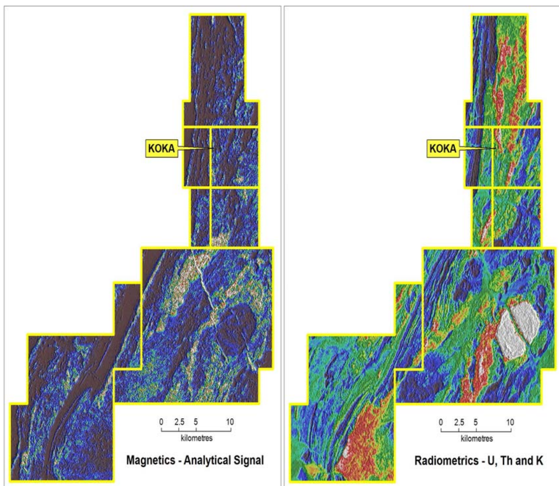
Figure 7: Aeromagnetic and Radiometric images, Zara & Hurum EL's
